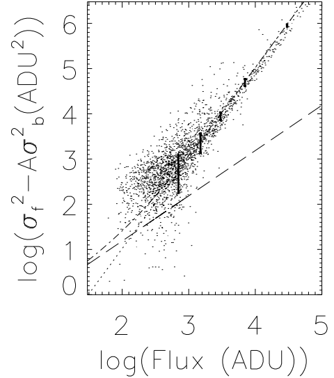
Figure 7. Comparison between the empirically calculated and model dispersions of the source fluxes. The term due to the local background noise is estimated in individual sources and is subtracted from the dispersions. The long dashed line and dotted line represent the model contributions from the Poisson fluctuation and the intrapixel sensitivity error, respectively, while the dash-dotted line represents their total contribution. Representative error bars are illustrated at five flux levels.
