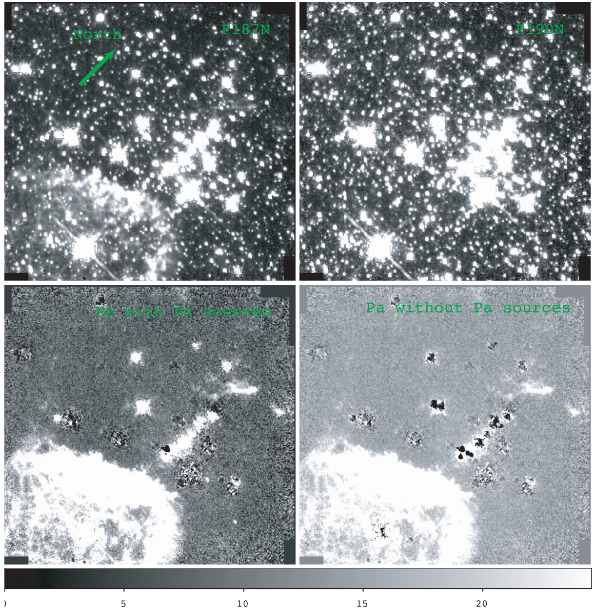
Figure 9. The F187N (upper left) and F190N (upper right) images and differenced images with and without Paschen \alpha -emitting sources (lower left and lower right, see Section 3.5) of the position ‘GC-SURVEY-72’ (in detector coordinates), which includes the central part of the Quintuplet cluster, the Pistol star and the Pistol Nebula. Diffuse Paschen \alpha emission from the Pistol Nebula dominates the Paschen \alpha images.
