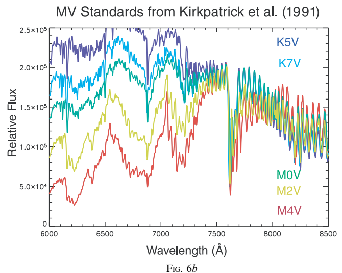
FIG. 6.—Spectral type of 2M1824. (a) The R = 4550 spectrum of 2M1824 from 2005 June 30. (b) Grid of M spectral standard stars, HD 190007 (K5 V), GL 786 (K7 V), GL 763 (M0 V), GL 806 (M2 V), and Barnard's star (M4 V). Using the spectral types assigned by Kirkpatrick et al. (1991), these standard stars bracket 2M1824AB and indicate a type of M2.5 Ve. We assign this spectral type to the brighter of the two stars.
