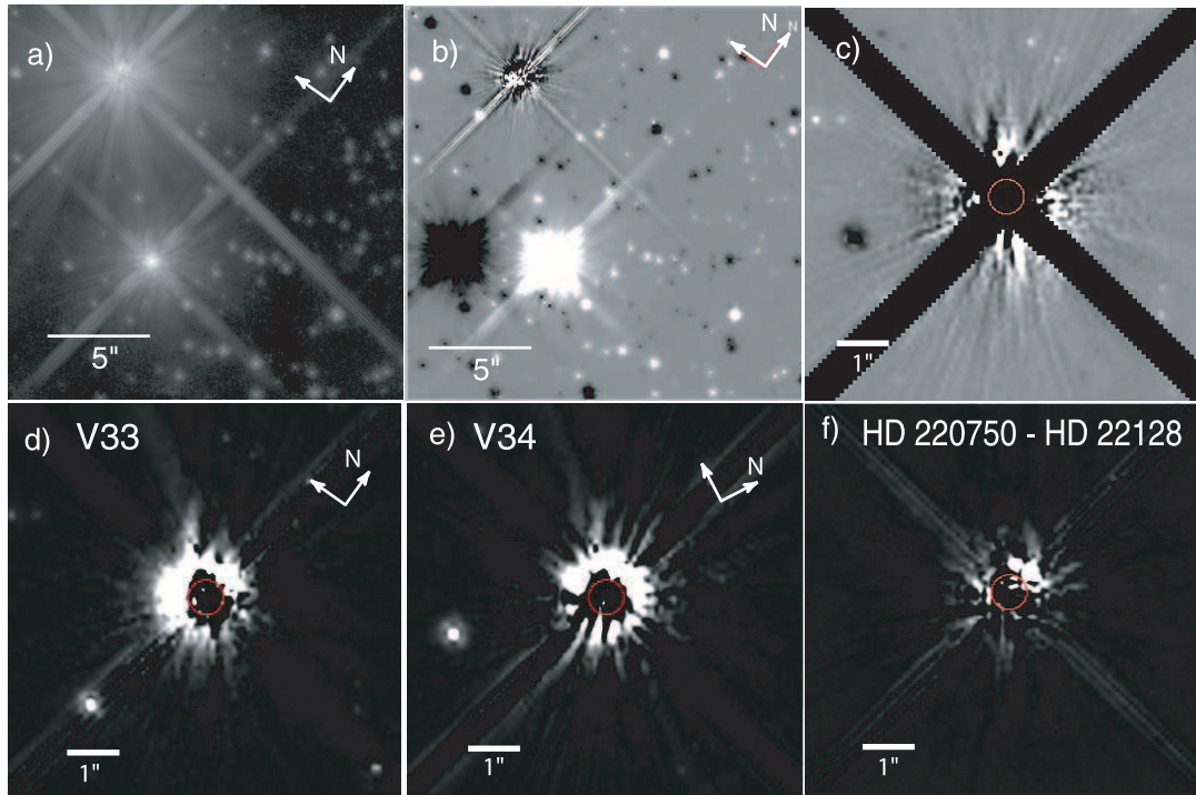
FIG. 1.—HD 169142 at 1.1\ \mu\text{m} (F110W) as seen by NICMOS. (a) The Herbig Ae star (upper left) and 2MASS 18242929–2946559 (2M1824) are the brightest objects in the 19.2'' \times 19.3'' NIC2 field of view. (b) Roll-differencing results in PSF subtraction residuals typical for the stability of the HST +NICMOS PSF, with no indication of nonaxisymmetric nebulosity. (c) Detail of the roll-differenced data showing both background stars at r \geq 2'' and the symmetric residuals typical of either a disk null detection or a face-on system. The data for (b) and (c) are shown with a linear stretch between -5 and 5 instrumental counts \text{s}^{-1}\ \text{pixel}^{-1} (ADU), which corresponds to a surface brightness range of \pm 1\ \text{mJy arcsec}^{-2} . After subtraction of color and breathing matched median PSF template observations, excess light is seen for (d) visit 33, (e) visit 34, and (f) at a level that is distinctly higher than for color-matched PSF subtractions. The data for (d, e) are shown with a linear stretch between 0 and 5\ \text{mJy arcsec}^{-2} , with white for \text{SB} > 1\ \text{mJy arcsec}^{-2} .
