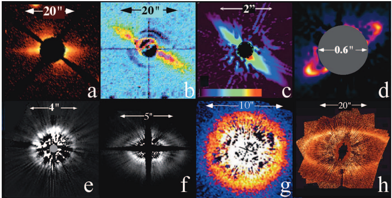
FIG. 15.— Circumstellar debris systems imaged in scattered light. (a) AU Mic; (b) \beta Pic; (c) HD 32297; (d) HR 4796A; (e) HD 181327; (f) HD 141569; (g) HD 107146; (h) \alpha PsA. See Table 3 for details. Fig. 15a reprinted with permission from Kalas et al., 2004, Science , 303, 1990; © 2004 AAAS. Fig. 15b reprinted with permission from Smith & Terrile, 1984, Science , 226, 1421; © 1984 AAAS.
