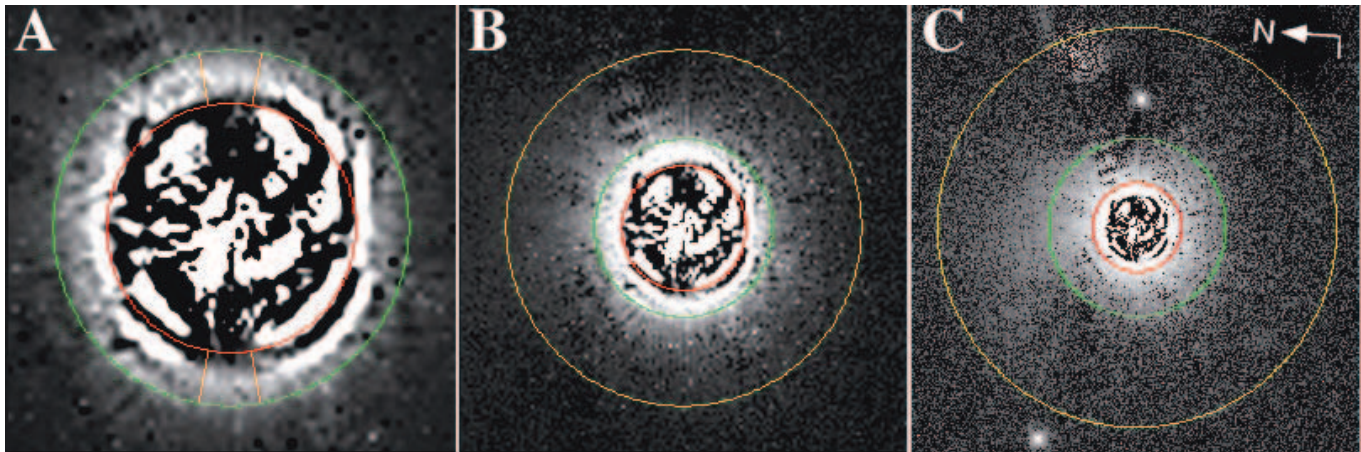
FIG. 3.— ACS 0.6 \mu\text{m} PSF-subtracted coronagraphic image of HD 181327. (a) 2.5'' \times 2.5'' field, r = 1.4'' (red), r = 2.0'' (green), -0.1 to +1.5 \text{ e}^- \text{ s}^{-1} \text{ pixel}^{-1} linear display. The disk is reliably seen only within \pm 10^\circ of the image +Y -axis (P.A. = 274.9^\circ ; arcs bounded in orange). (b) 5'' \times 5'' field, r = 1.4'' (red), r = 2'' (green), r = 4'' (yellow), 0 – 1 \text{ e}^- \text{ s}^{-1} \text{ pixel}^{-1} square root display. (c) 10'' \times 10'' field, r = 2'' (red), r = 4'' (green), r = 9'' (yellow), [-3.3] to [+0.0] \text{ e}^- \text{ s}^{-1} \text{ pixel}^{-1} logarithmic display. Within \pm 45^\circ of north and 4'' – 9'' from the star a faint nebulosity can be seen, with some suggestion of curvature toward the east.
