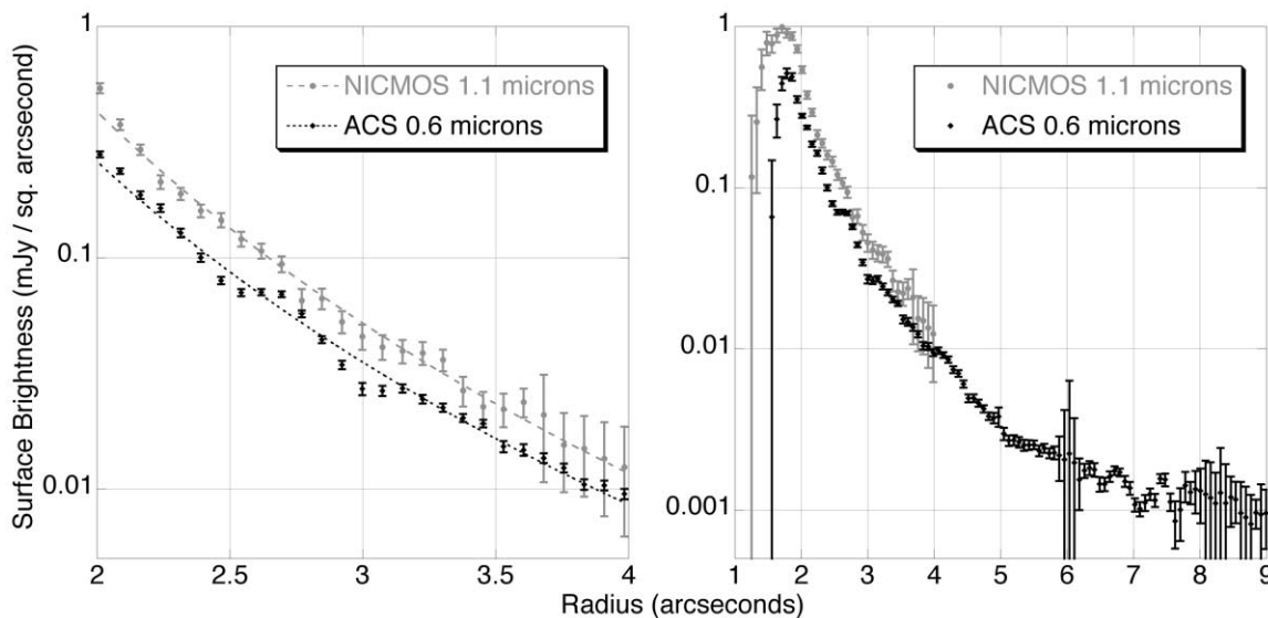
FIG. 8.— NICMOS and ACS deprojected SB profiles of the HD 181327 circumstellar disk from (left) 2''–4'' (~100–200 AU) and (right) inner detection radii to 9'' (~450 AU). NICMOS profile is limited to r < 4'' due to field of view truncation (see Fig. 9) and integration depth. The 1\sigma error bars are the standard deviations of the measured SB in each 1 pixel wide radial zone about the zonal median and do not include uncertainties in the absolute calibration of the disk flux densities. The ACS profile was measured after resampling the image to the NICMOS pixel scale (effectively smoothing the image with an \approx 3 pixel \times 3 pixel kernel).
