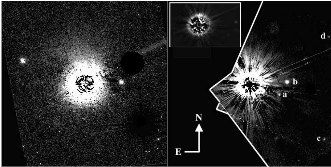
FIG. 9.— Outer regions of the HD 181327 disk in (left) the ACS and (right) the NICMOS PSF-subtracted images within \pm 12''.5 of the central star. Both images are square root displays with maximum intensities (hard white) corresponding to 1.4 \text{ instrumental counts s}^{-1} \text{ pixel}^{-1} . Four stars common to both fields are noted (denoted a–d). Inset: Debris ring revealed in the NICMOS image, shown at the same spatial scale and image orientation (linear display from -0.25 to +10 \text{ counts s}^{-1} \text{ pixel}^{-1} ).
