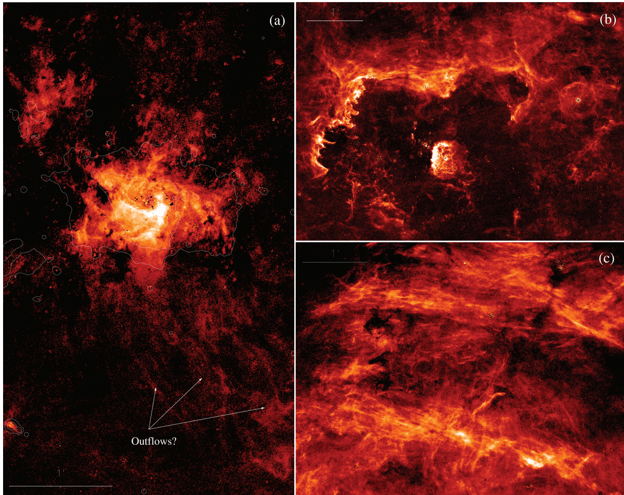
Figure 4. Close-ups of the P\alpha -emitting features: (a) the central region around Sgr A*, with overlaid IRAC 8 \mu m intensity contours at 1, 3, 10 and 30 \times 10^3 mJy sr ^{-2} ; (b) the Sickie nebula [G0.18–0.04; e.g. (Lang, Goss & Wood 1997)] and (c) thermal Arched filaments (e.g. Lang, Goss & Morris 2001). All are projected in the Galactic coordinates.
