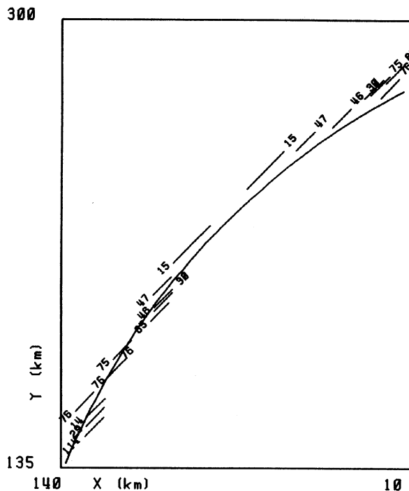
Fig. 8. Pallas profile (5 of 9). A steep slope is defined on the reappearance (left) side by stations 47 to 65. The valley that produced the short reappearance for station 76 is in the lower left part of the figure. A 50 km crater might explain this topography. A second slope is traced by the final reappearance at stations 76 and 114. The topography is clearest in this area near the northern limit, where the effects of visual timing errors are minimal. See also Fig. 13.
