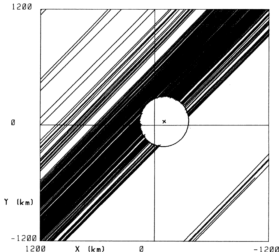
FIG. 14. Sky plane observed around Pallas.
