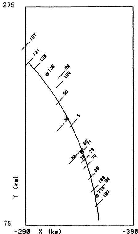
FIG. 4. Pallas profile (1 of 9). Photoelectric and video observers are indicated with a circle; visual timing error bars are shown by short lines (see Sec. V). The station numbers are given for each.
