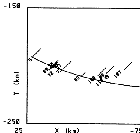
FIG. 12. Pallas profile (9 of 9).
