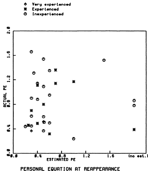
FIG. 17. Personal equation at reappearance.
