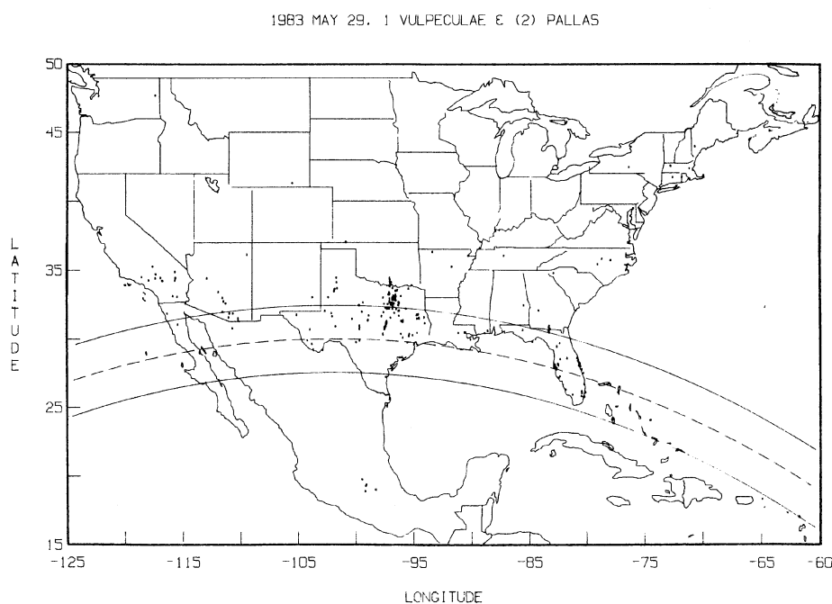
FIG. 1. Path of the occultation. Observation sites are shown with dots. All reported observations from the western hemisphere were from the continental U.S. and Mexico.
