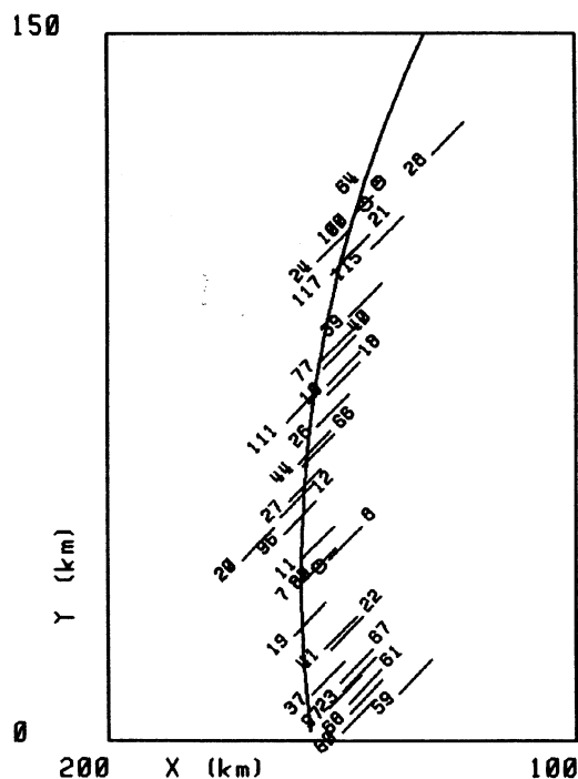
FIG. 9. Pallas profile (6 of 9). Stations 39 to 96 ( r = +95 to +45 ) seem to show a slight increase of elevation towards the south. From station 96 to the bottom, the elevation decreases significantly.
