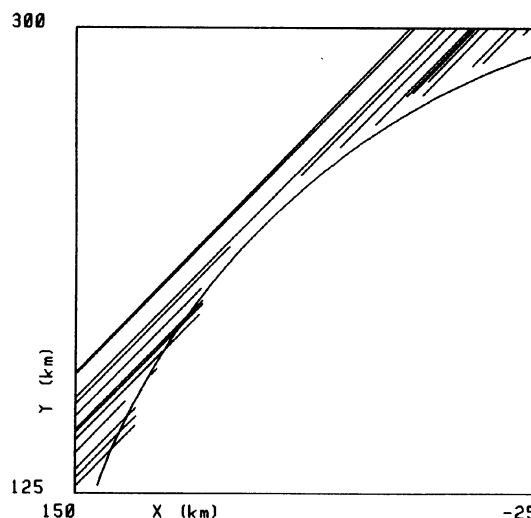
FIG. 13. Northern cap observations. The lines indicate when the star was seen, interruptions when it was occulted. The three miss stations plotted are 317 (closest to the asteroid), 206, and 209.
