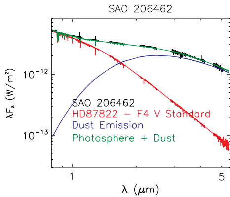
Figure 3. Model for SAO 206462. The SED consists of the underlying photospheric emission of the star plus thermal emission by the inner dust ring. The relative strengths of the two components were adjusted to match the observed continuum emission of the star plus disk system.
