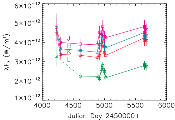
Figure 4. Time variability of the near-IR continuum for all 13 epochs. The outburst in 2009 seems to have appeared first in the J -band, and is similar to the “high- J ” state described by Grady et al. (2009). We have set the uncertainties on the data at all but the first epoch at 7%, which are propagated into the line flux measurements; the agreement among the various flux-normalization sets is often much better. The AAVSO photometry and SpeX Prism data on February 18 agree to better than this precision. The uncertainty in the first epoch was set to a generous 15% because no independent flux calibration data was available for it. As no LXD spectrum was obtained on 2007 July 8, there is no L -band flux plotted for that date.
