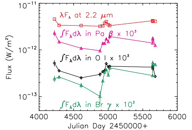
Figure 8. Time variability of Paschen \beta , Br \gamma , O I 0.8446 \mu\text{m} , and the K band for all 13 epochs.
