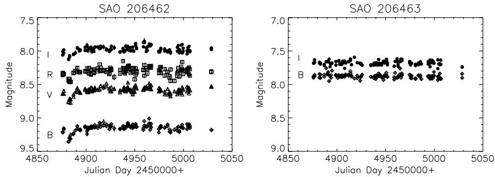
Figure 1. Left: BVR photometry of SAO 206462 (HD 135344B), obtained in 2009 with the 35 cm telescope of the Sonoita Research Observatory, operated in part by the AAVSO. The point-to-point scatter is dominated by scintillation and atmospheric changes. Longer-term modulation is possibly due to star spot activity. The drop in brightness seen near JD=2454880 days is consistent with the lower flux level derived from the SpeX Prism data in 2009 February 18. Right: photometry of SAO 206463 (HD 135344A), the A0V star located 22 arcsec from SAO 206462, and based on the same photometric calibration. For clarity, only the data in the B and I filters are shown. The flux drop seen in SAO 206462 is not seen here, conforming its reality for the other star.
