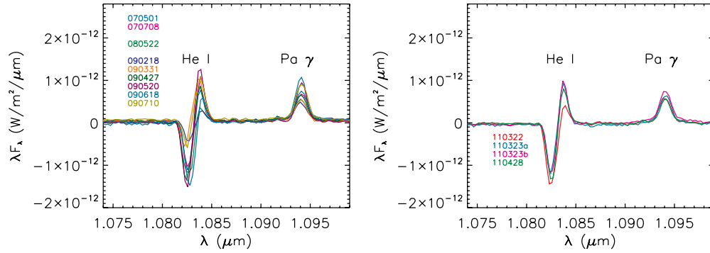
Figure 7. Left: flux-calibrated continuum-subtracted He I 1.08 \mu\text{m} and Paschen \gamma lines for all nine epochs between 2007 and 2009. As in Figure 6, the Pa \gamma line exhibits a small amount of epoch-to-epoch shifts in central wavelength, but here is less than one resolution element. In contrast, the He I line, with a wind-dominated profile, exhibits much greater variability. Right: the same lines during 2011. The two sets of data from March 23 were obtained only 2 hr apart, and are nearly identical. The He I line changed significantly between March 22 and 23.
