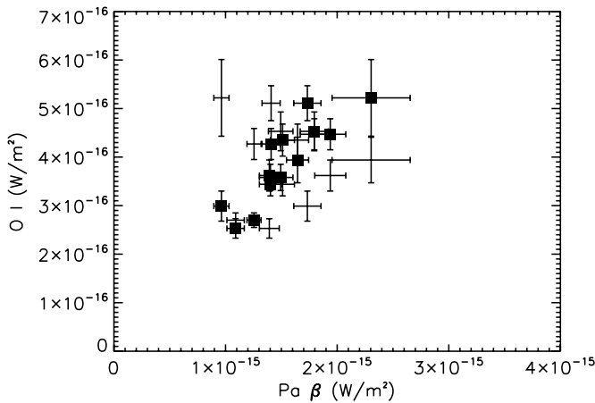
Figure 10. Relative strengths of Pa \beta and O I \lambda 8446. The filled symbols represent the actual observations, with matching dates of observation. The data shown only as error bars represent the same data set “rotated” by three epochs, to illustrate in a simple manner the result of using two non-simultaneous data sets.
