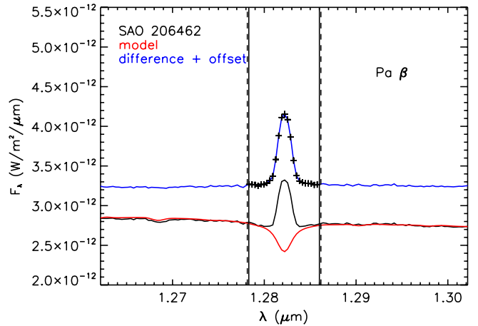
Figure 5. Line extraction for Paschen \beta for 2009 July 10 UT. Here the difference between the observations and the model is offset for clarity. The vertical lines and the plus symbols indicate the wavelength range over which the net line strength was measured.
