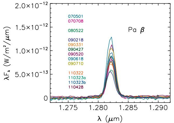
Figure 6. Flux-calibrated continuum-subtracted Paschen \beta for all 13 epochs. The “jitter” in the central wavelength is likely dominated by a combination of the spectral sampling and uncertainties in the wavelength calibration.
