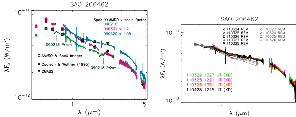
Figure 2. Left: SAO 206462 observed on three epochs in 2009, illustrating the absolute calibration process. Also shown are archival 2MASS data, which seem to have been obtained during a state similar to that to May 20, and BVRJHKLM photometry from Coulson & Walther (1995), when SAO 206462 was in a “steep spectrum” state similar to that of March 31. Right: the SpeX XD data obtained in 2011 March were normalized using REM photometry obtained within 1–2 days of the spectra. In the 5 days of photometry obtained in March, SAO 206462 was photometrically stable. Additional photometry obtained in May indicated that the emission from the inner dust disk had declined (the beginning of another “steep spectrum” event), but the VRI emission levels indicated that this was not due to changes in the stellar photospheric brightness at these wavelengths.
